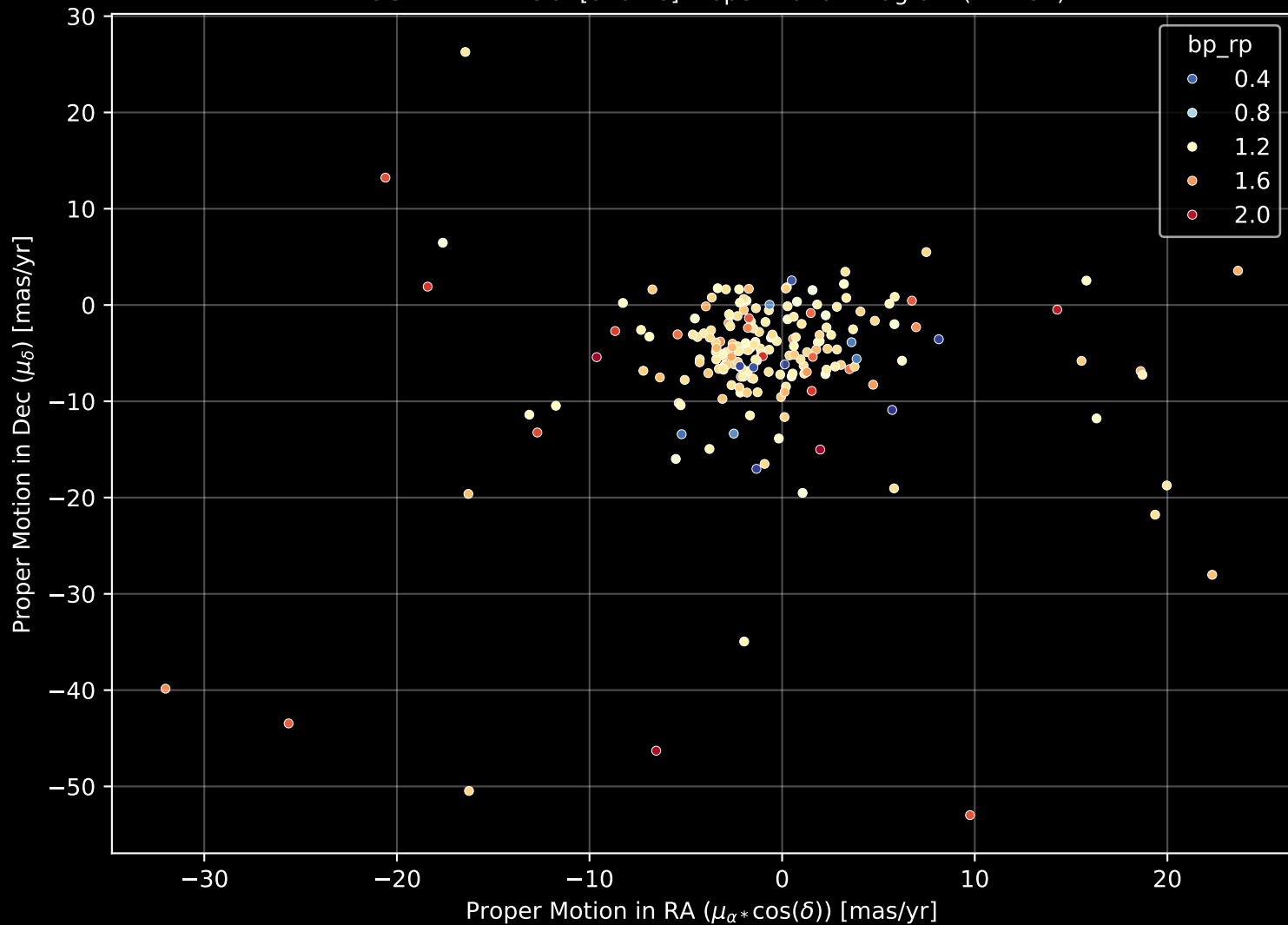
APOGEE DR17 Field: [020-16] Proper Motion Diagram (n= 197)
