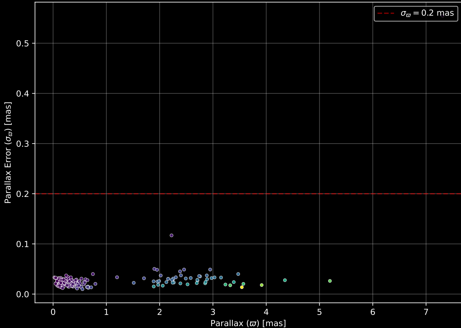
APOGEE DR17 Field: [020-16] Parallax Quality (n= 197)
