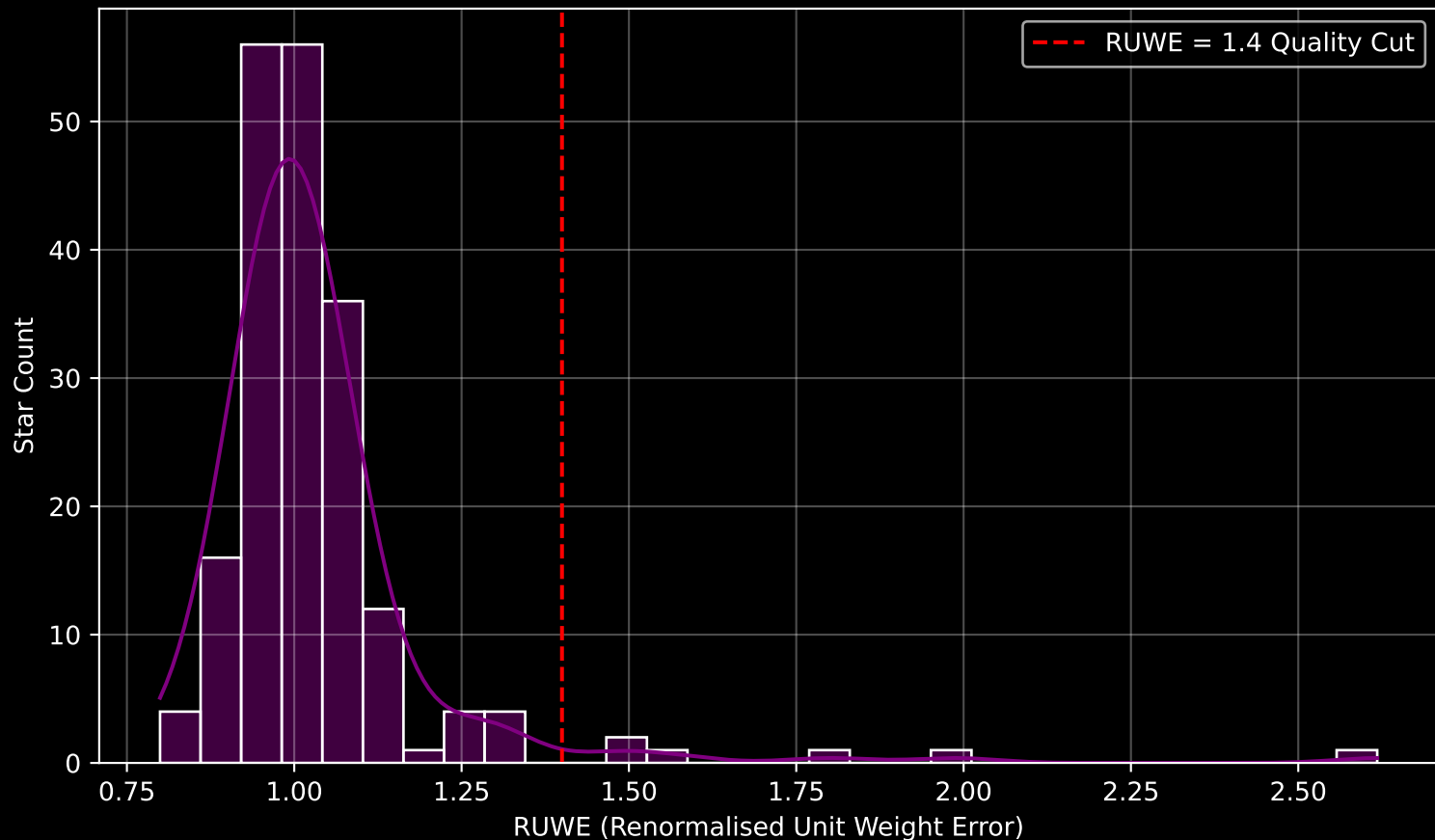
GAPOGEE DR17 Field [020-16] RUWE Distribution (n= 195)
