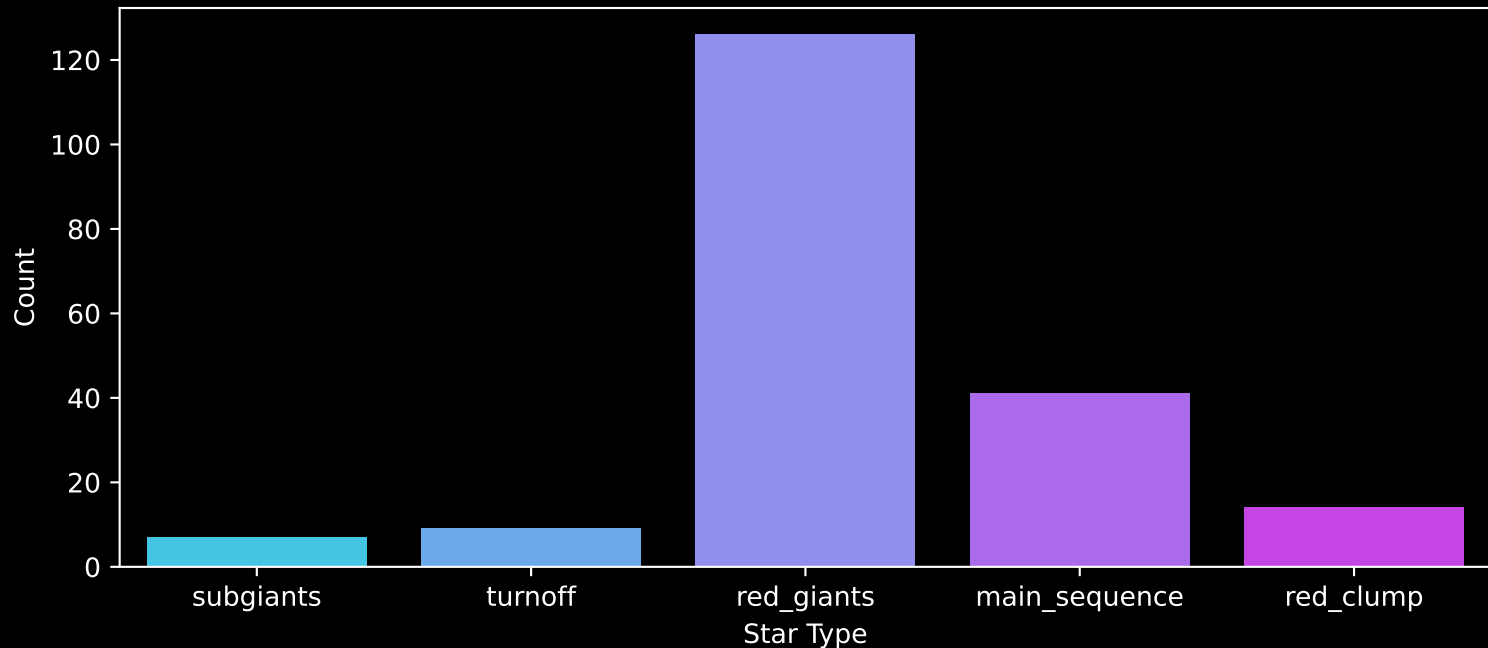
APOGEE DR17 Field: [020-16] Count plot of Star Type
