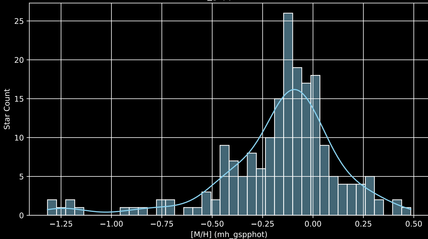
APOGEE DR17 Field: [020-16 [M/H] (mh_gspphot) (n= 196)
