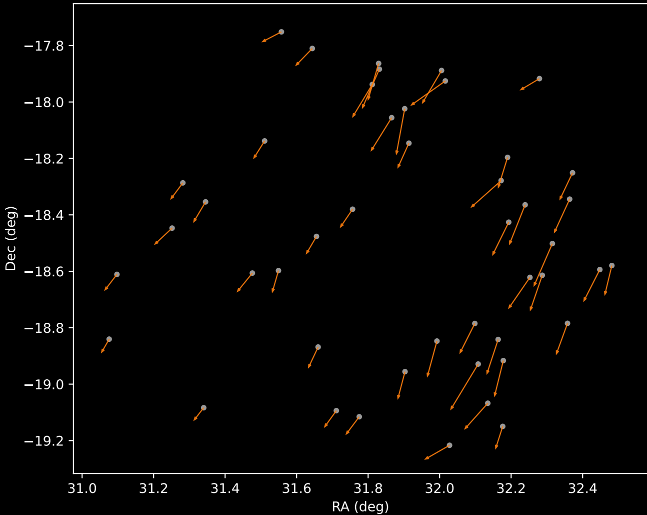
APOGEE DR17 Cluster 2 Proper Motion Vectors (n=46)
